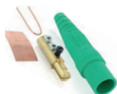
Enchufe (male) c/2 pernos t/Cam Type 400A 600V C:2/0-4/0 16D24-G
